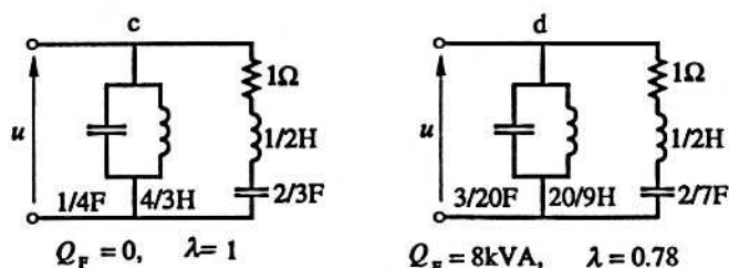
Fig. 8a-d. a,b Two loads that cannot be distinguished in terms of Frizz's powers. c,d The same loads with reactive compensators that improve power factor to maximum value
