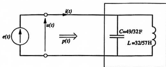
Fig. 2. Circuit with zero Budeanu's reactive power Q_B but with energy oscillation
