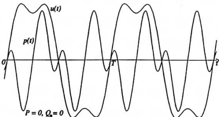
Fig. 3. Supply voltage u(t) and instantaneous power p(t) in the circuit shown in Fig. 2. At negative values p(t) energy flows to the supply source
