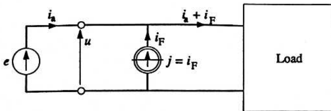
Fig. 9. Circuit with Fryze's reactive current i_F compensated by controlled current source
