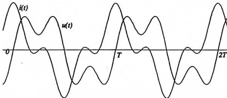
Fig. 6. Mutual distortion of the voltage and the supply current in the circuit shown in Fig. 5. with zero distortion power D
