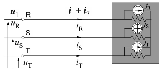
Fig. 7. Resistive balanced HGL generating the 7 th order current harmonic
