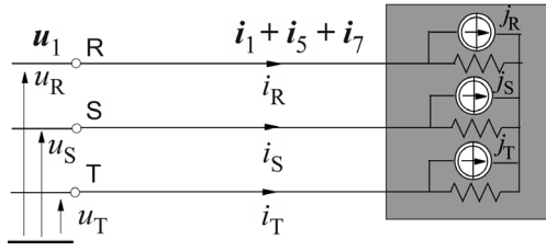
Fig. 8. Resistive balanced HGL generating the 5 th and the 7 th order current harmonic
